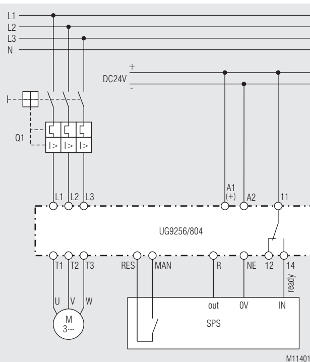
Motor control with UG 9256/804 and PLC
